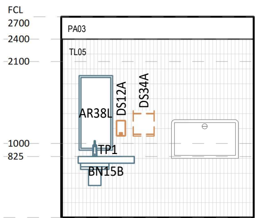
2 ELEVATION DETAIL 1 : 50
