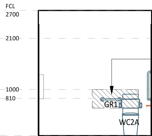
3 ELEVATION DETAIL 1 : 50
