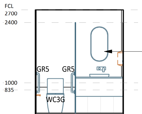
7 ELEVATION DETAIL 1 : 50
