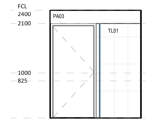
9 ELEVATION DETAIL 1 : 50
