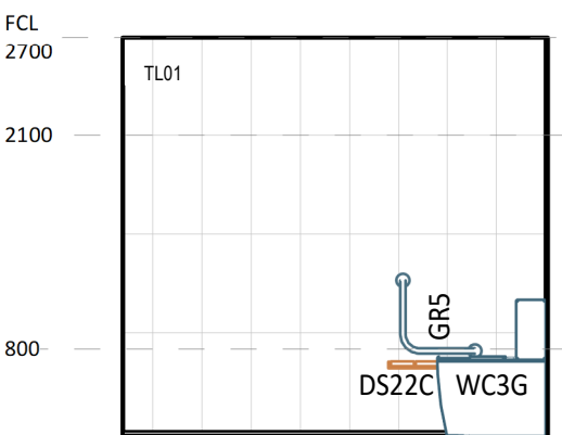
6 ELEVATION DETAIL 1 : 50
