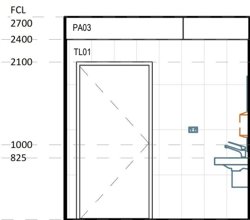
5 ELEVATION DETAIL 1 : 50
