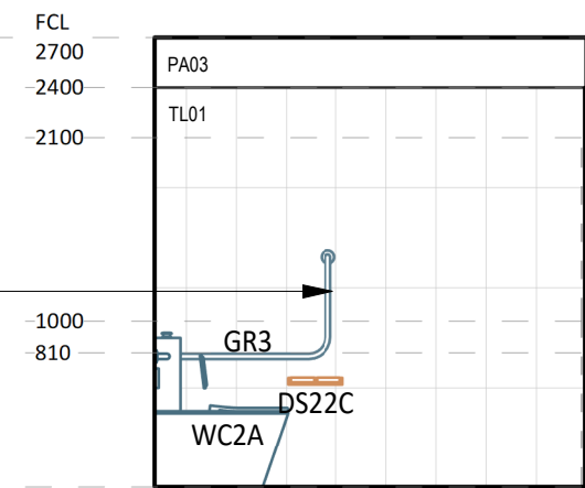
4 ELEVATION DETAIL 1 : 50
