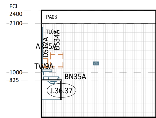
8 ELEVATION DETAIL 1 : 50
